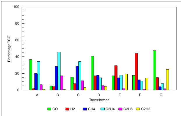
Figure 1: DGA signatures for faulty transformers
