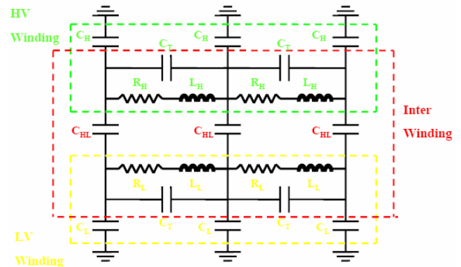
Figure 1: Simplified equivalent circuit with lumped RLC components
