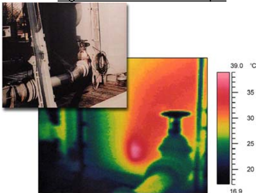
Figure 3: IR scan of a hot spot
