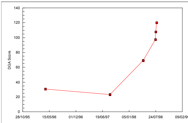
Figure 2: DGA score for core earth fault
