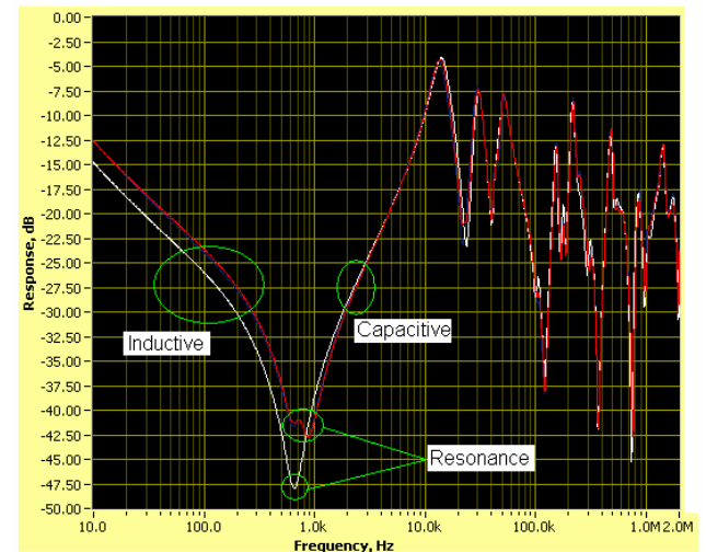
Figure 2: Frequency Response of a sound transformer
